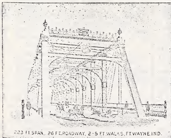
223 FT SPAN. 26 FT. ROADWAY, 2-5 FT. WALKS, FT. WAYNE, IND.
